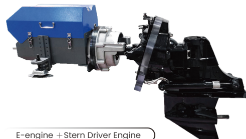
E-engine + Stern Driver Engine
